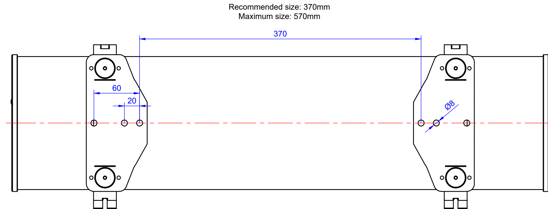
Bottom View
